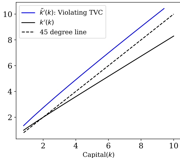
Figure 14: Comparison between the optimal solution, denoted by k'(k) , and a solution that violates the transversality condition, denoted by \tilde{k}'(k) , in the recursive neoclassical growth model. The solution that violates the transversality equation intersects with the 45 degree line at \tilde{k}_{\max} \approx 30 .
