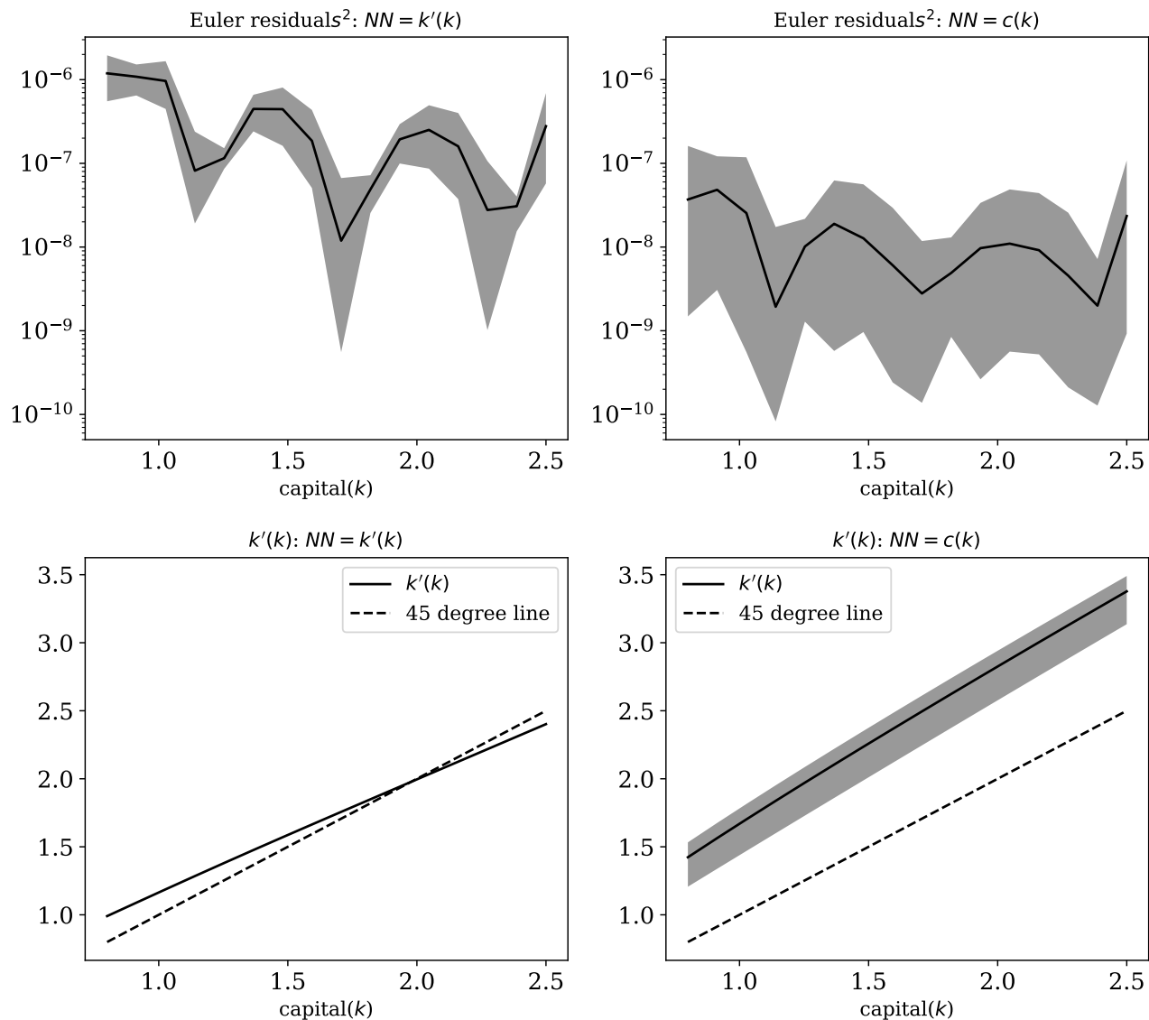
Figure 15: Comparison between approximating the policy function for capital k'(k) versus the consumption function c(k) with a deep neural network. The left panels show the median of Euler residuals and policy functions for capital when k'(k; \theta) is approximated with a deep neural network. The right panels show the median of Euler residuals squared and policy functions for capital when c(k) is approximated with a deep neural network. The solid curves show the medians and the shaded regions show the 10th and the 90th percentiles over 100 different seeds.
