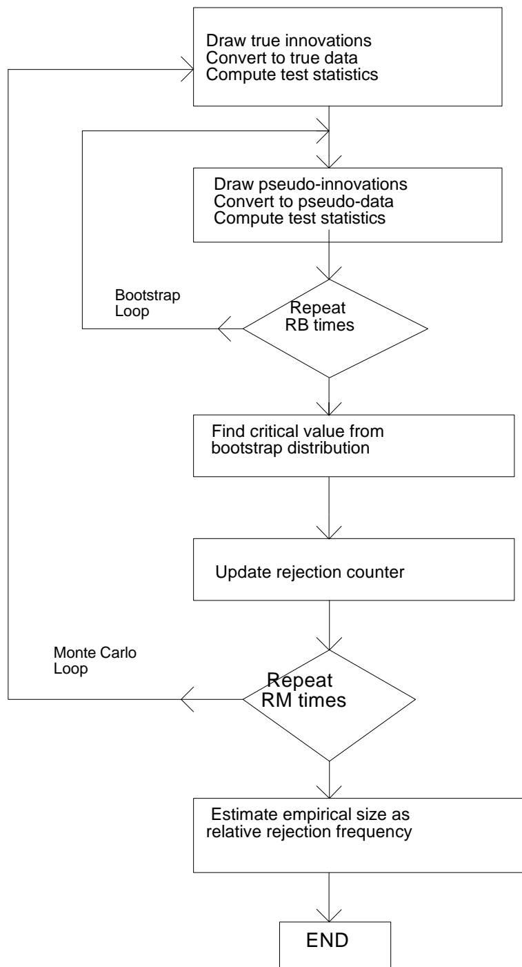
Figure 5 Flow Chart for Bootstrap Monte Carlo
