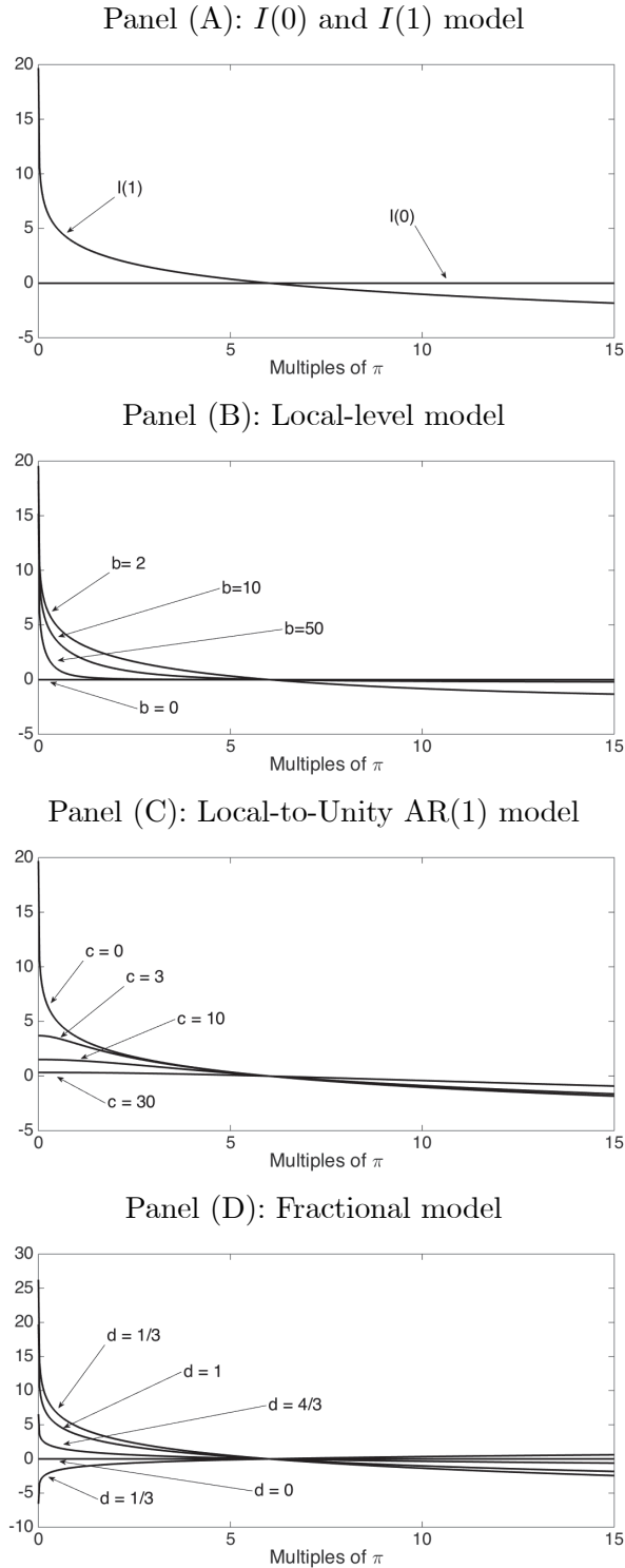
Figure 13: Local-to-Zero Log-Spectra of some Benchmark Models of Low-Frequency Variability
