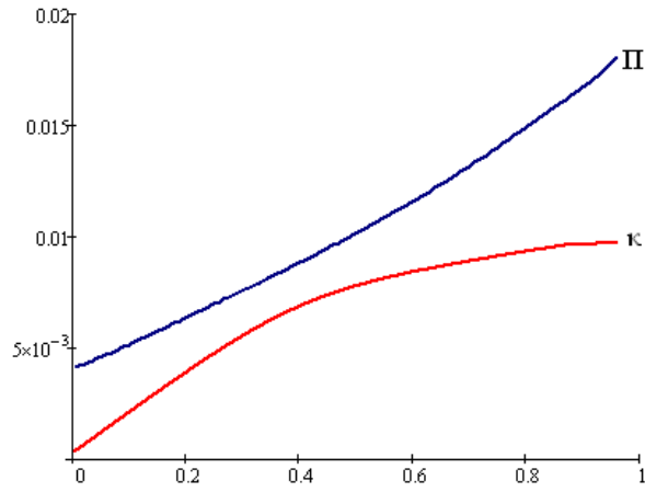
Figure 3: \rho^* = 1
