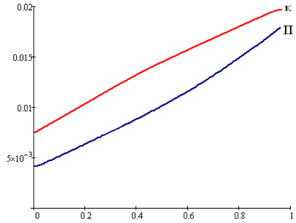
Figure 4: \rho^* = 0
